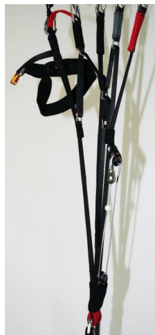
Fig 3 AGERA RS riser
